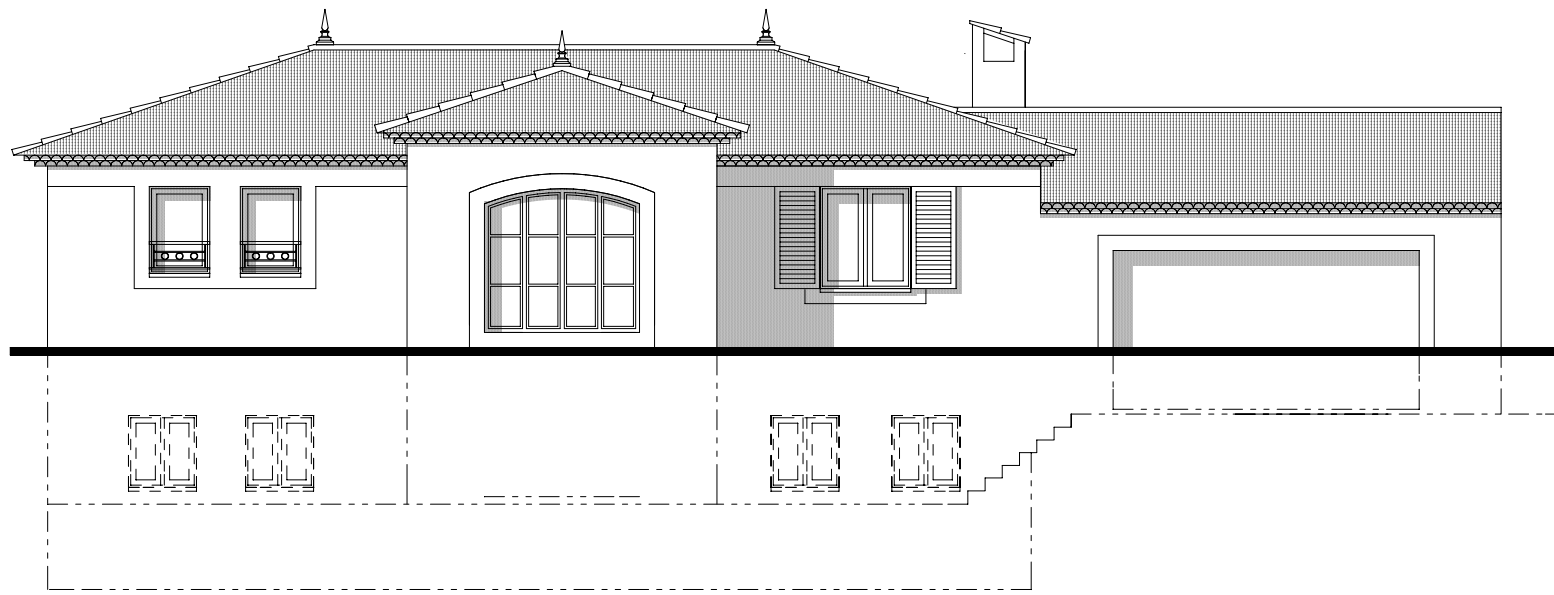
FACADE ENTREE
